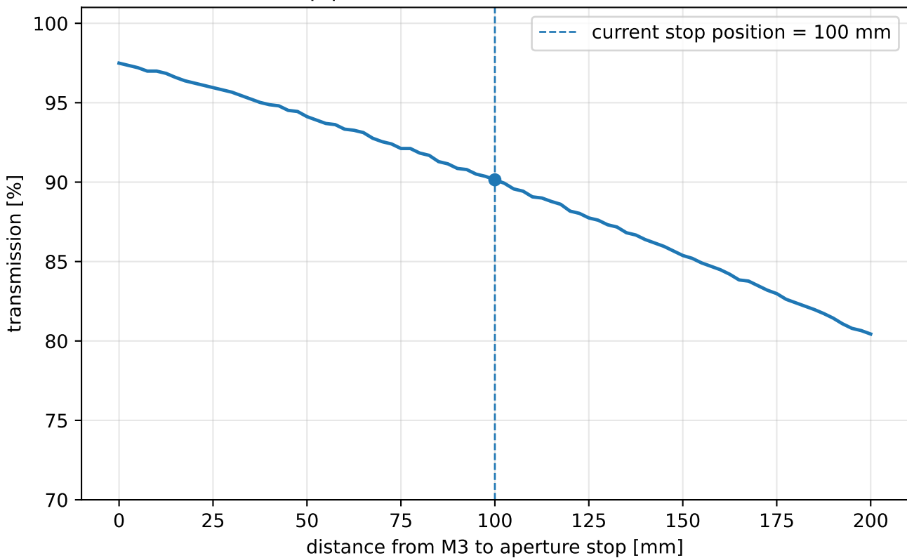
Transmission vs. stop position, field = +1.22^\circ , theta = 0 (the worst case)
